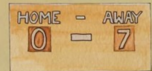
loss
